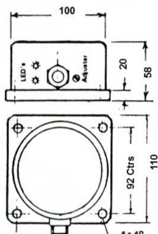
TYPE MD 22100-55 Nominal Range 55mm
