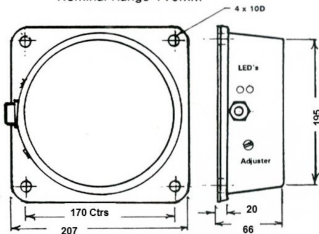
TYPE MD 22200-110 Nominal Range 110mm
